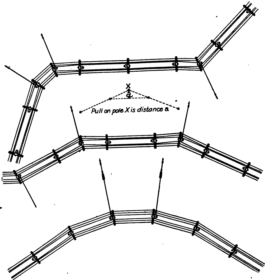
FIG. 121.—Method of guying on curves.
